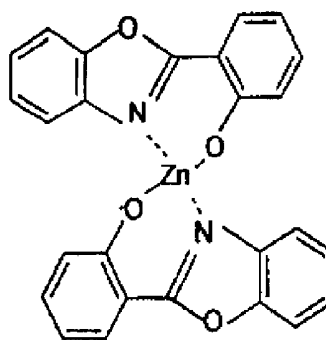
ZnPBO
