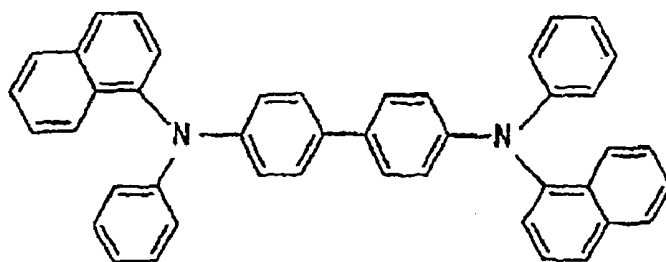
\alpha -NPB
