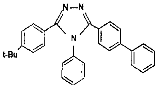
TAZ
