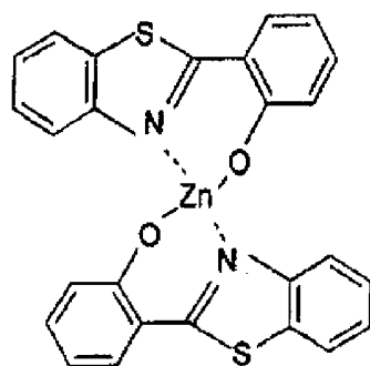
ZnPBT
